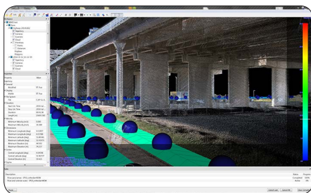
Point cloud and image locations
