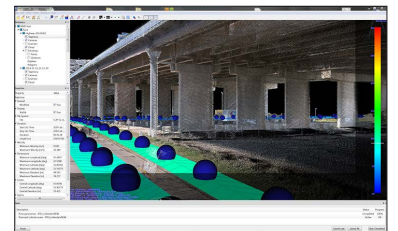
Multiple lasers provide optimum coverage
